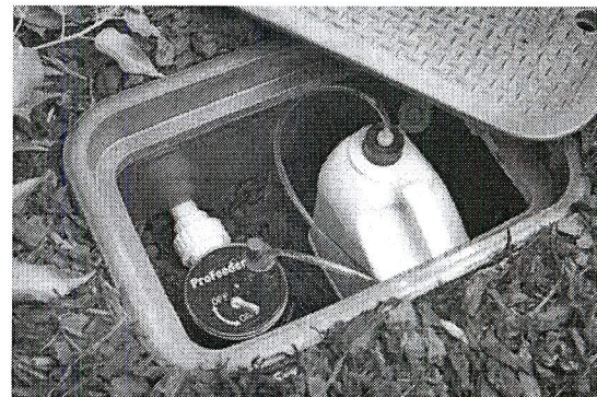
Figure 5: A properly installed ProFeeder will look something like the illustration above. Notice that the valve box has been placed in the opposite direction of the irrigation system piping to make plenty of room for the fertilizer bottle. A jumbo valve box may also be used to accommodate larger fertilizer bottles for larger landscapes.
